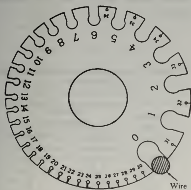
FIGURE 4-82. A wire gage.
